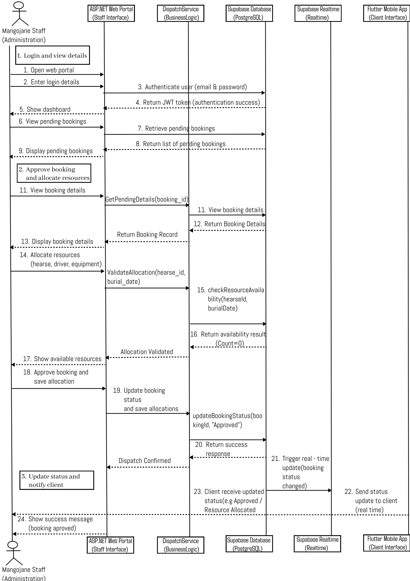
Sequence Diagram 2: Approve Booking and Allocate Resources (ASP.NET Web Application)
